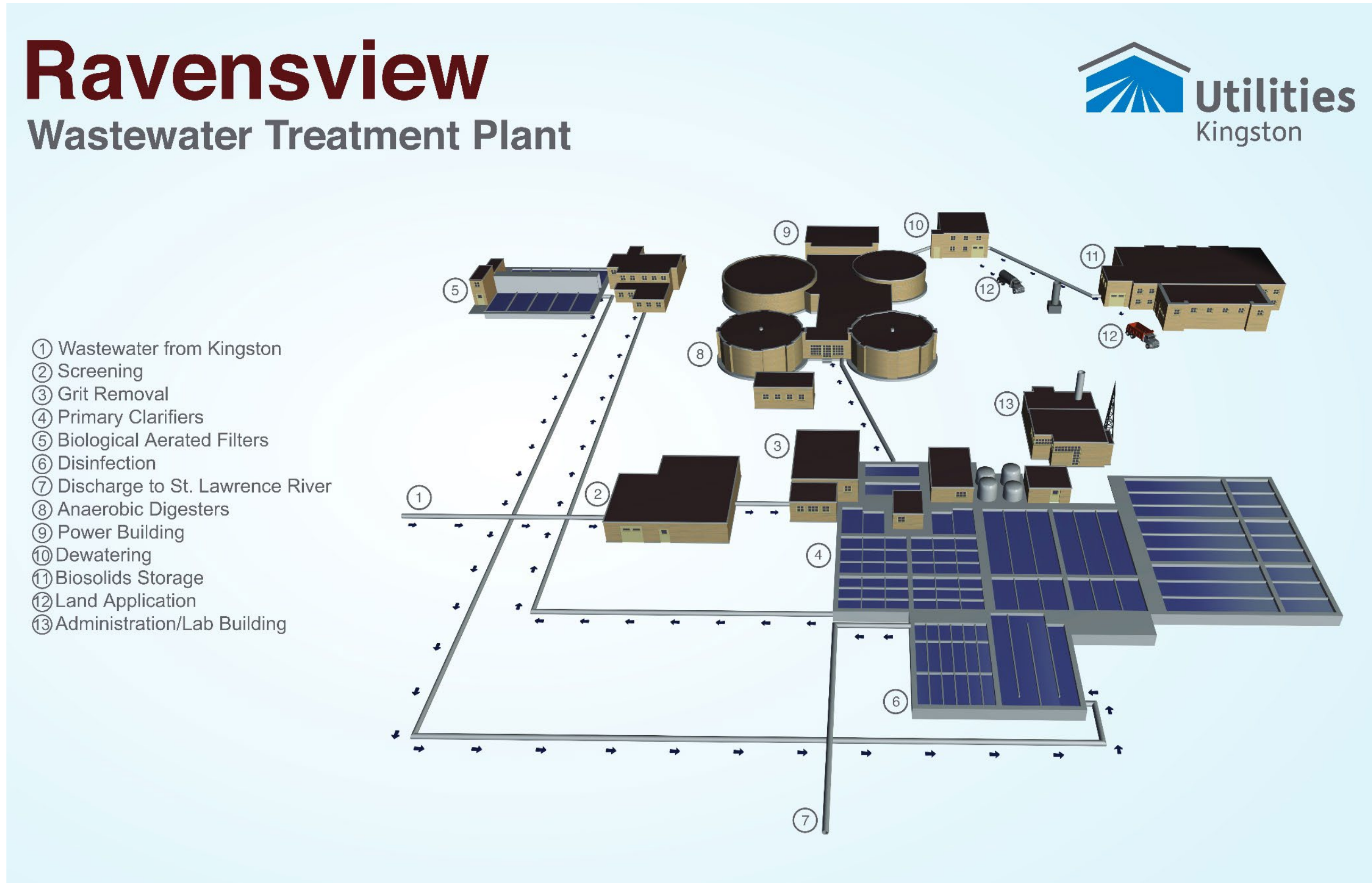
Figure 1 - Ravensview Water Pollution Control Plant General Layout
